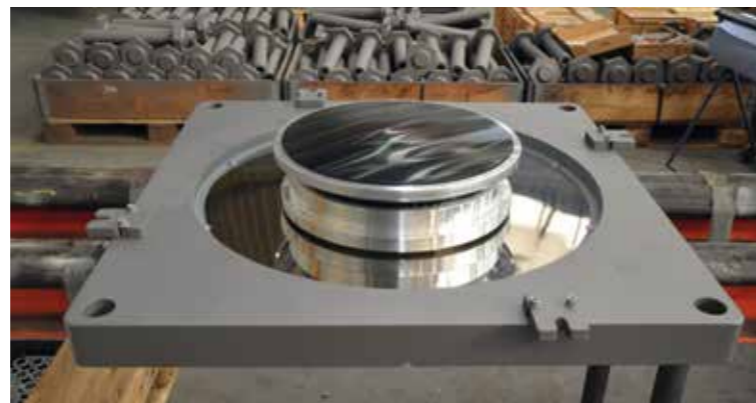
Lower sliding surface with articulated slider
